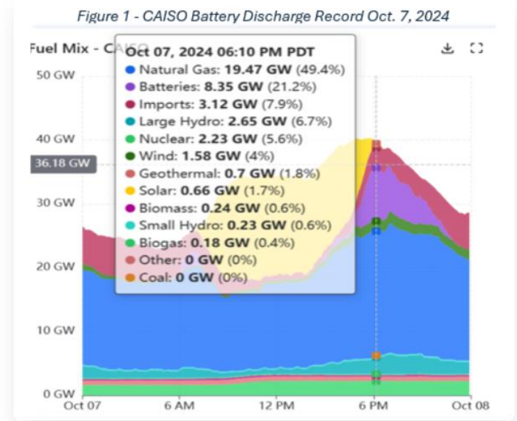
Figure 1 - CAISO Battery Discharge Record Oct. 7, 2024
