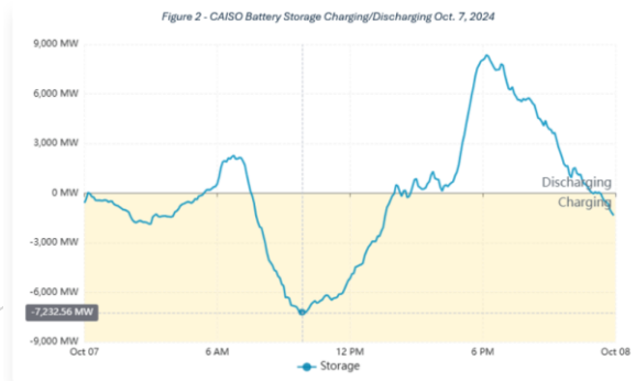
Figure 2 - CAISO Battery Storage Charging/Discharging Oct. 7, 2024
